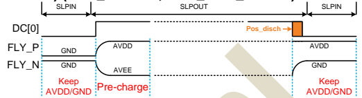
Case 4) (VGH_PWS=H ; VGH_PWS_GND=H)
