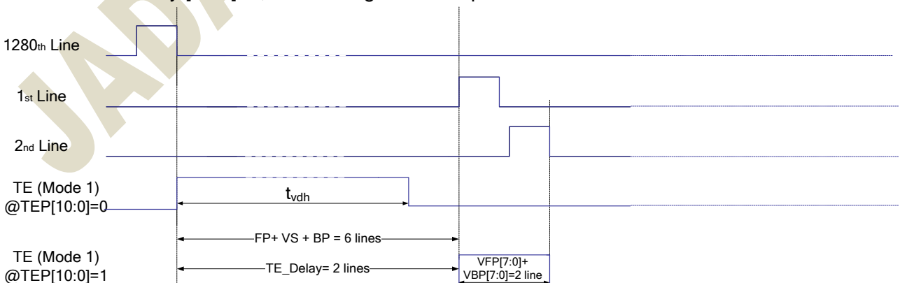
Figure 9.2: TE Line Delay under mode 1
