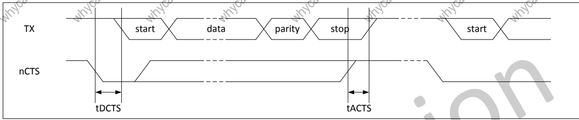
Figure 5-17 UART nCTS Timing
