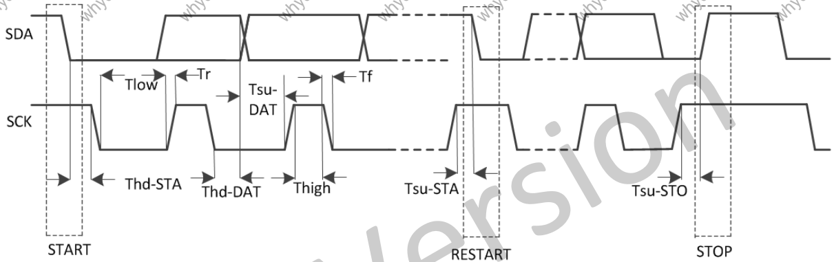
Figure 5-19 TWI Timing
