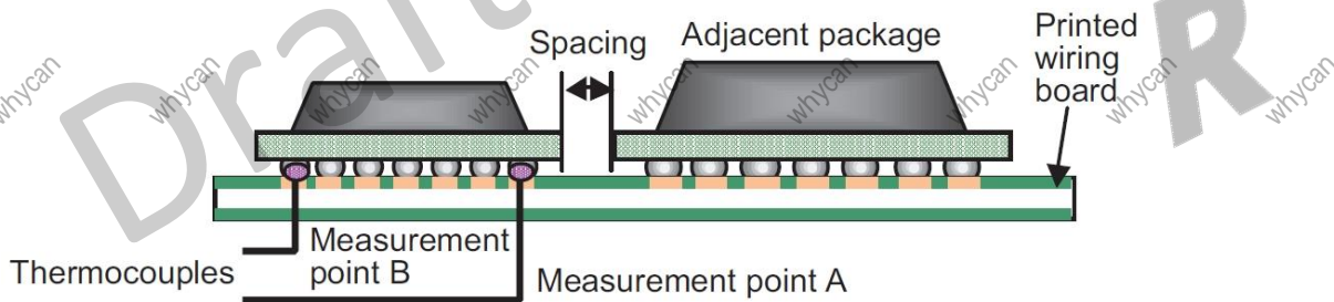
Figure 9-2 Measuring the Reflow Soldering Process
