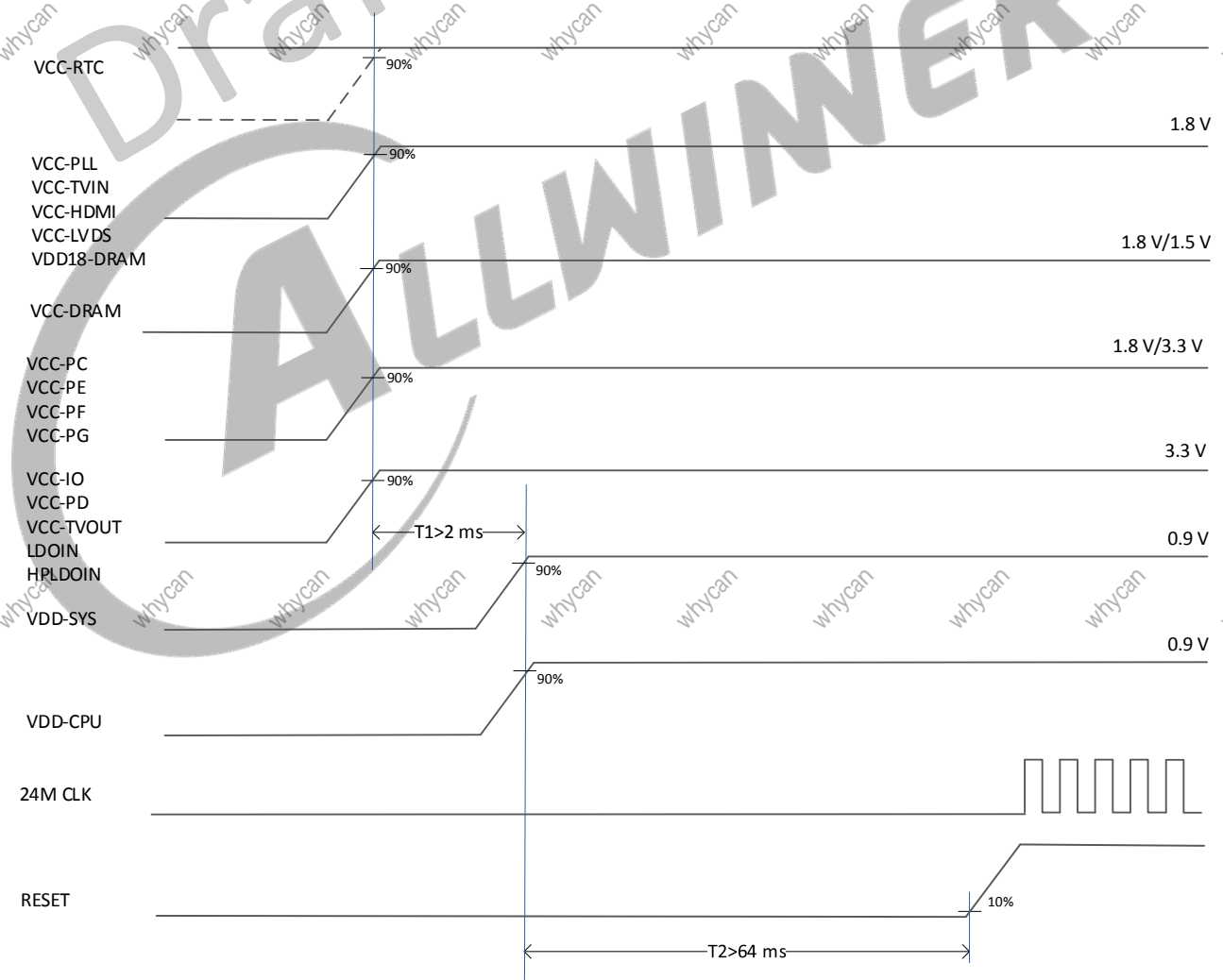
Figure 5-25 Power-On Timing
